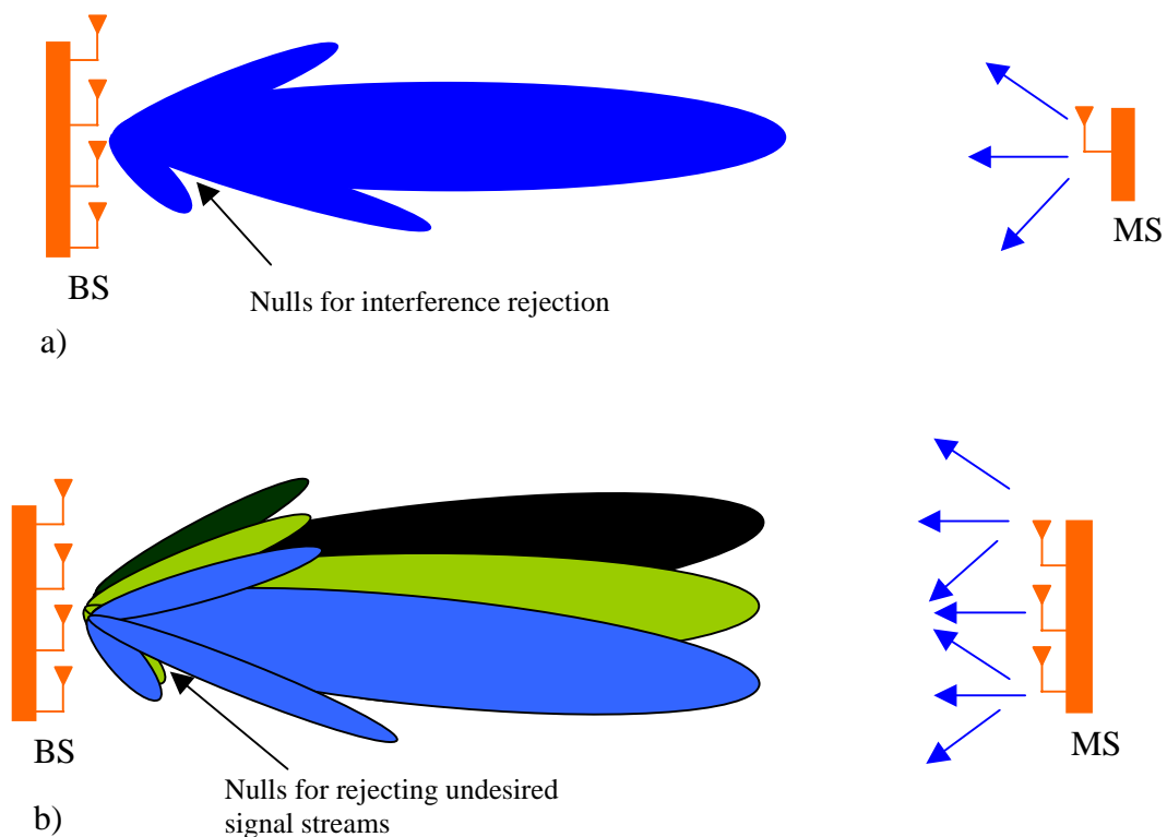
Figure 2: Uplink Antenna Systems a) BS Antenna system with K=1 and L>1 . b) MIMO antenna system with K>1 and L>1 .
