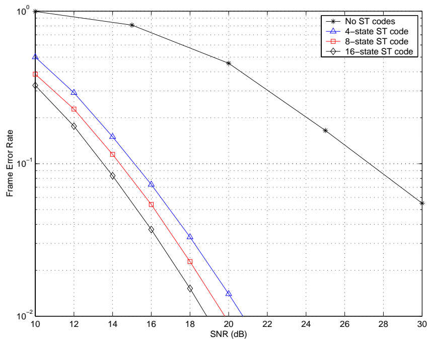
Figure 7: Performance of QPSK space-time (ST) codes over a flat Rayleigh fading channel with two transmit and one receive antennas and a frame size of 130 symbols.
