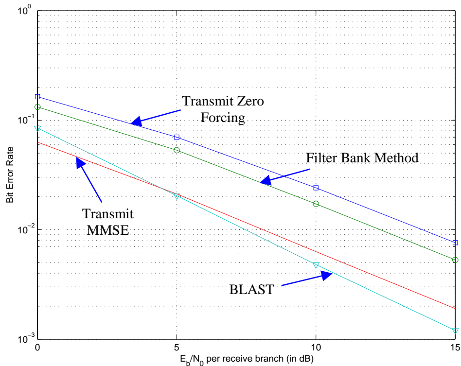
Figure 8: Performance Comparison of various MIMO transmitter based MIMO systems when M=N=4 .
