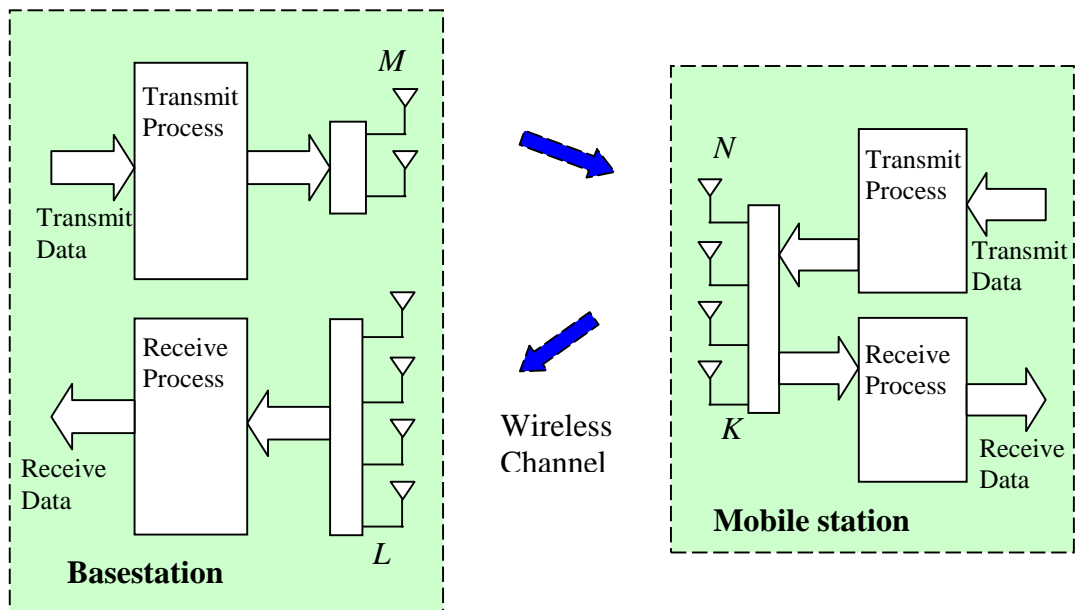
Figure 1: General Antenna System for Wireless Broadband Communications
