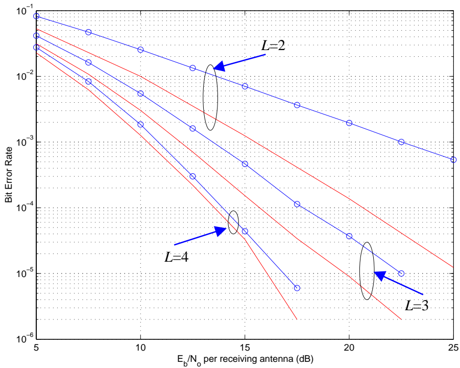
Figure 6: Performance comparison between MLD (solid lines) and BLAST (circled lines) with two transmit antennas ( K=2 ) and various numbers of receive antennas (in this case L ) with QPSK modulation.
